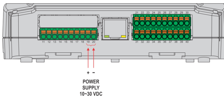
Figure 11 – Power supply
