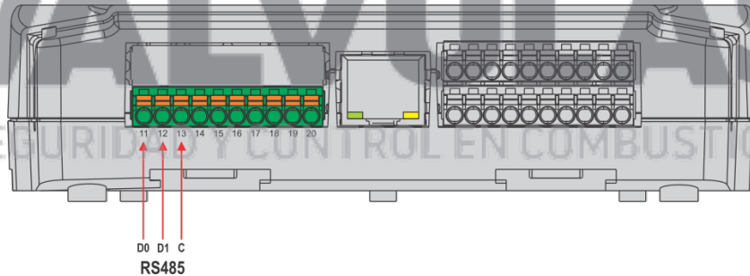
Figure 17 – RS485
