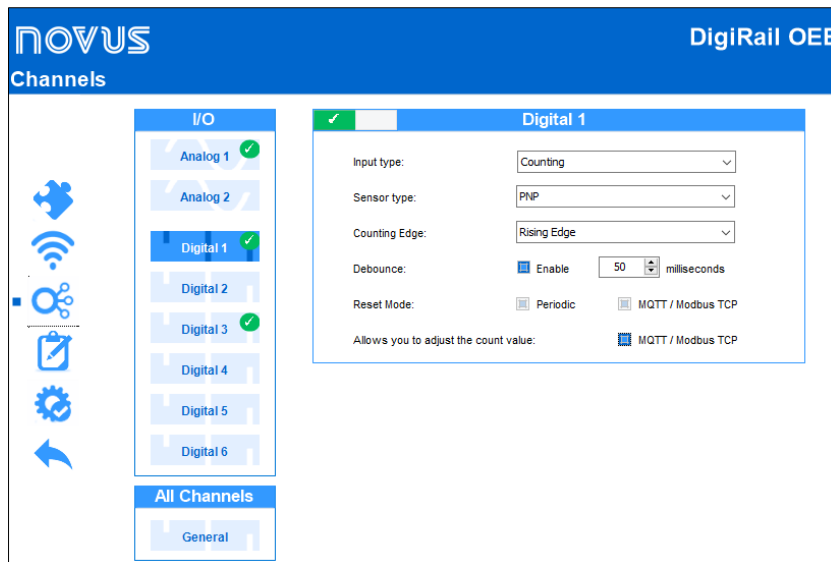
Figure 28 – Digital channels
